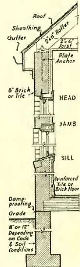
Wall Section
